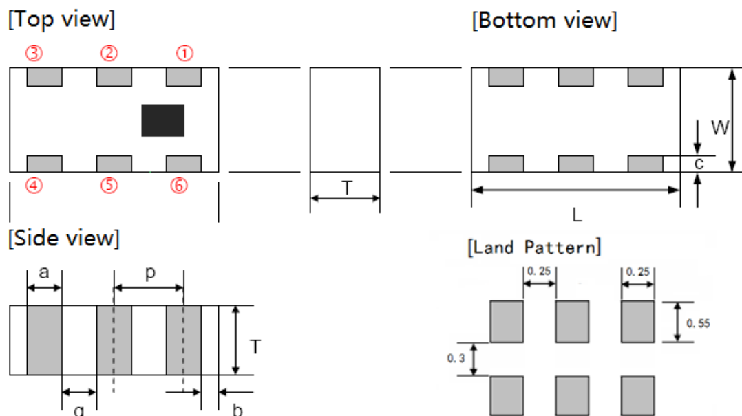
PIN Configuration
